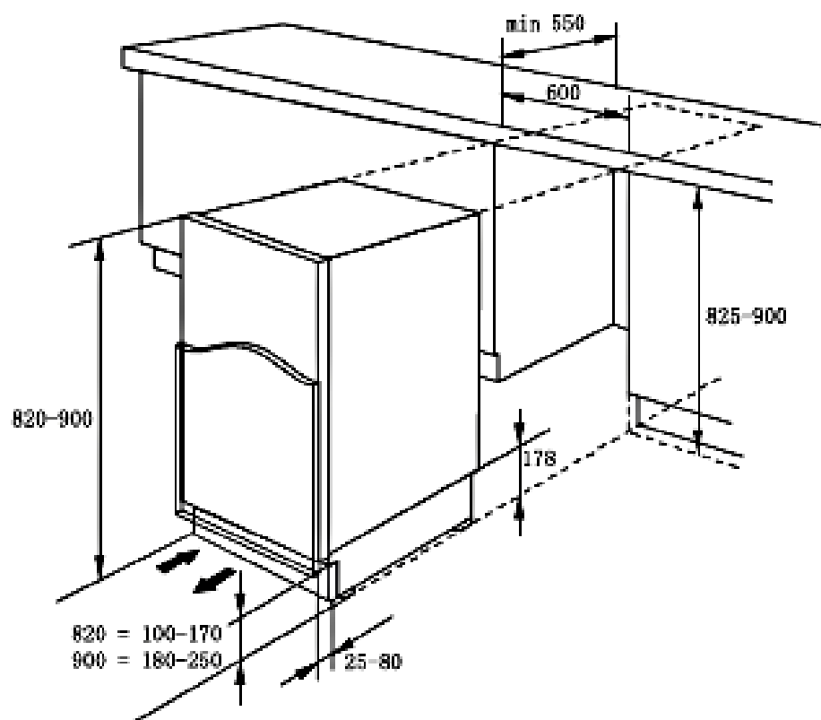
Fig 1 -Dimensions of mounting slot
