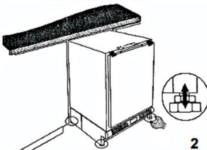
Fig 2 -Height regulation
