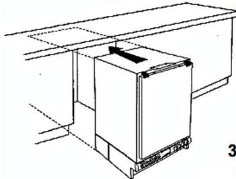
Fig 4 -Fastening the appliance under the worktop
