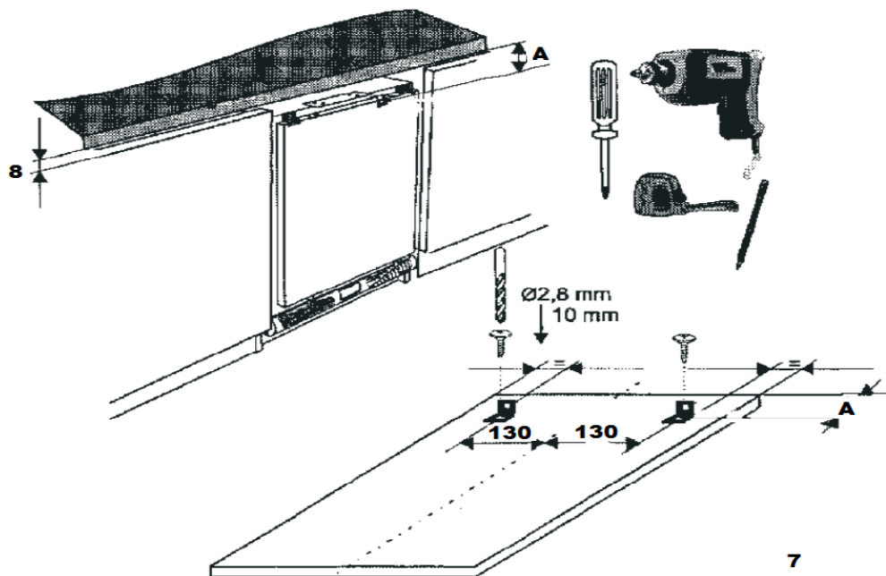
Fig 7/8 – Mounting the kitchen cabinet door
